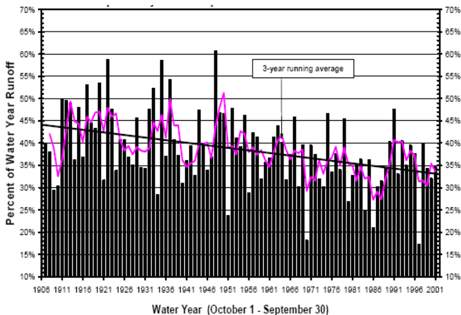
Figure 5.9-7 Sacramento River runoff in percent of Water Year runoff
